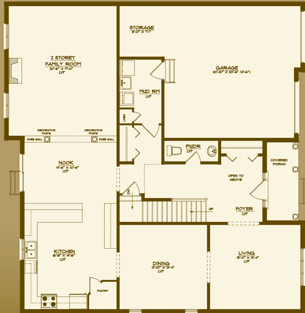
Main Floor 1,658 Sq. Ft.
